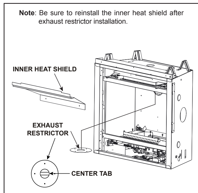
Figure 4.13 Exhaust Restrictor Installation
